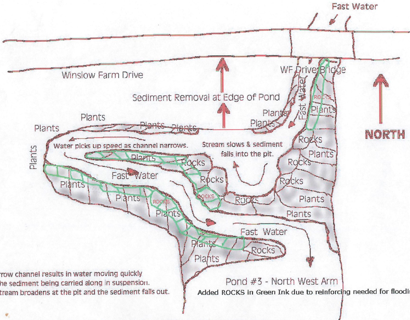
Water-Garden plus Sediment Pit at Bridge Inlet to Pond Three
